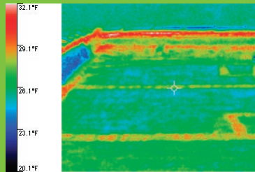
Cool areas on this roof exposure probably indicate moisture buildup. Mark with tape and investigate with core samples.
